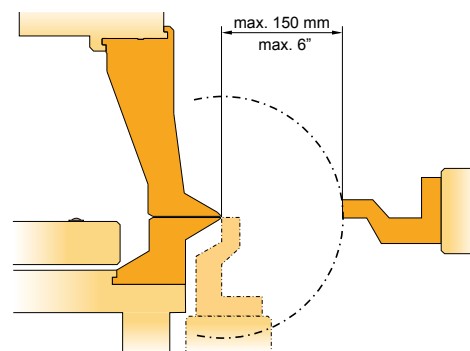
Folding beam travel range when folding direction changes
