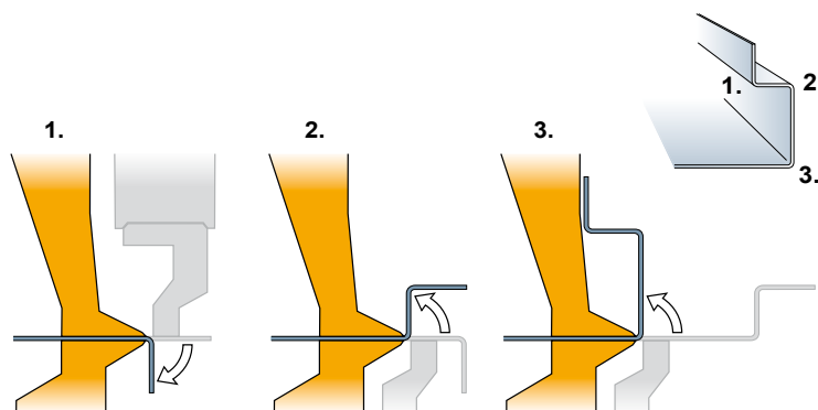
Folding sequence mostly from the outside in
