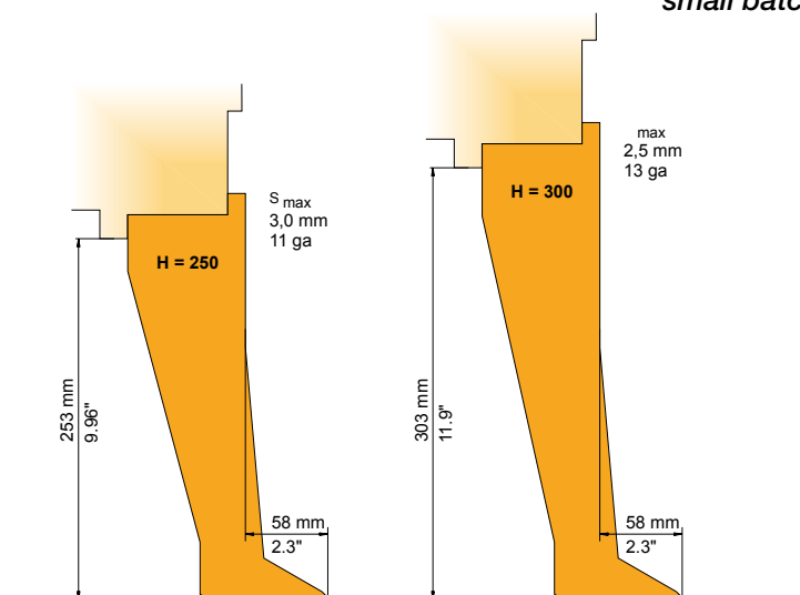
Tools for Upper Beam (left) und Folding Beam (above)
