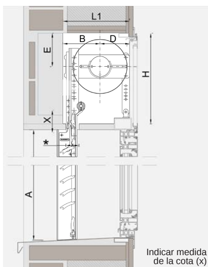
Enrollamiento interior
