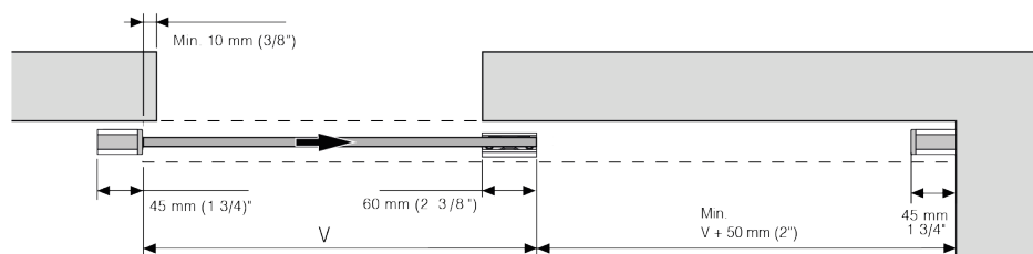
KSC Unikglass+ 50/100V ≥ 800 mm (31 1/2")
