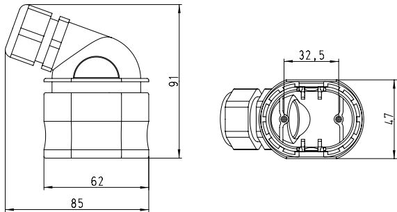
Hood 10-pole + ground side cable entry
