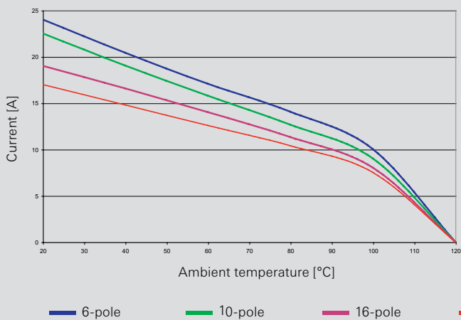
Derating curve according to IEC 60512 sec. 3 revosBASIC crimp version 500V / 16 A / 1.5 mm 2
