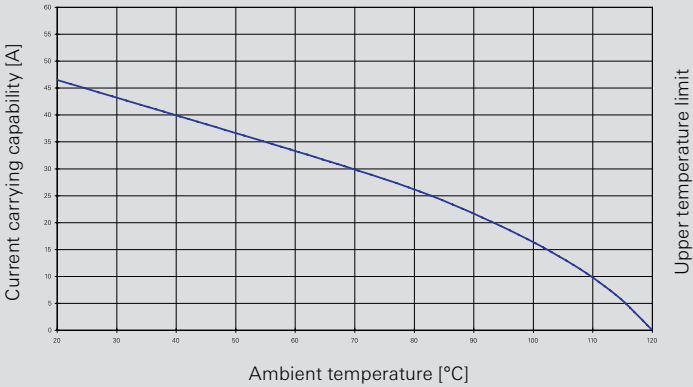
Derating curve according to IEC 60512 sec. 3 72.205/215.1253.0 revos POWER 6+6-pole 690 V / 400 V / 230 V 40 A / 16 A / 10.0 mm 2 / 2.5 mm 2
