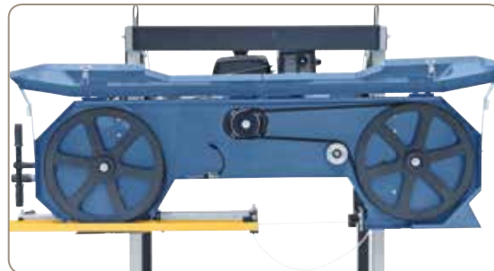
Tiltable covers allow for easy bandsaw blade change.
