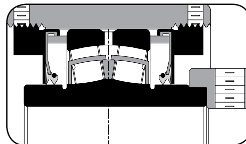
Fig. C-27. Double-lip seals.
