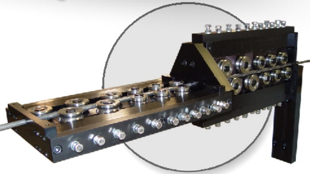
Dual Size Straightener Rollers for Wide Range of Wire Diameters
