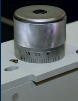
Standard: Manual blade gap adjustment, two-sided
