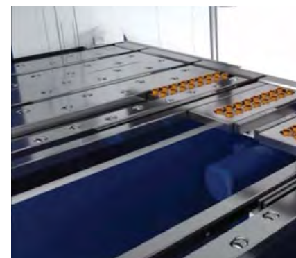
U-gauge with balls in table and suction gauge for smooth handling of the sheet
