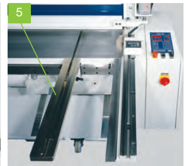
Movable sheet support with T-slots on linear guide
