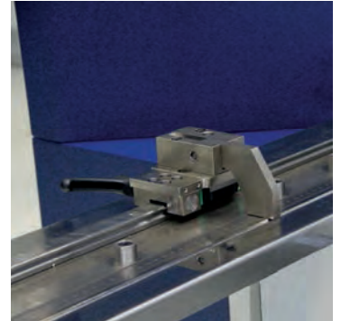
Option: lateral side gauge on linear guide rail incl. automatic tipping gauge
