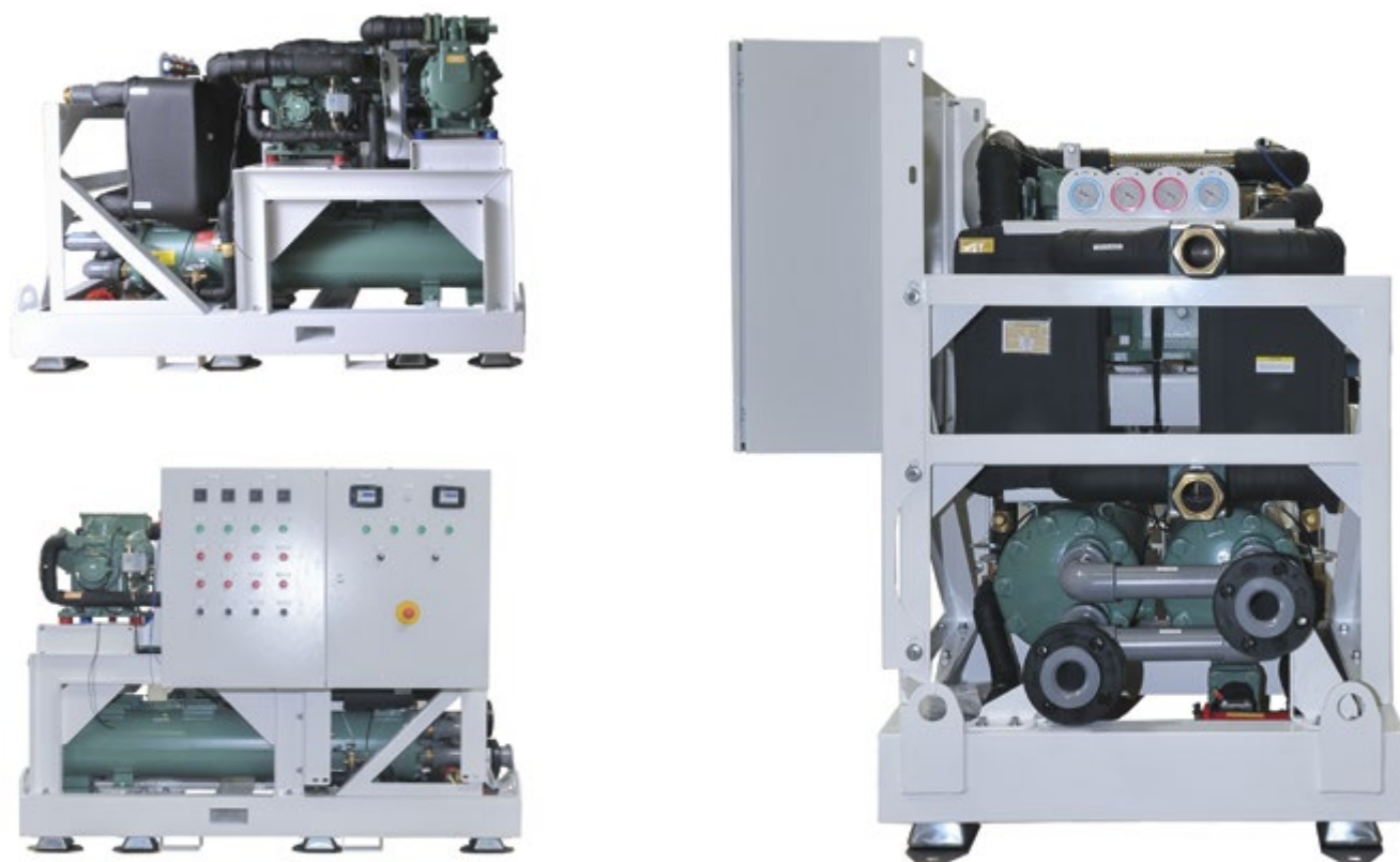
Examples of a 2-stage Q-Series high capacity chiller unit
