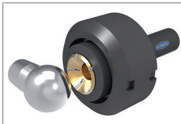
Roller burnishing a ball with type RKAK
