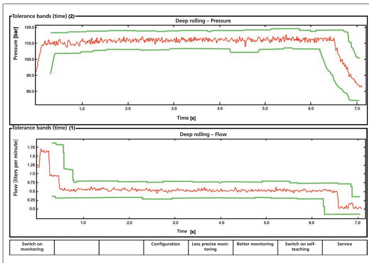
Process monitoring with tolerance bands
