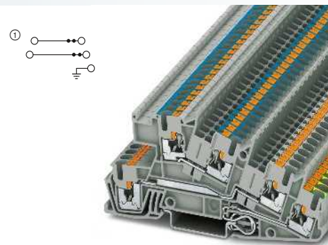
30 A, borne de tres pisos, 1 conductor exterior L, 1 conductor N, 1 PE
