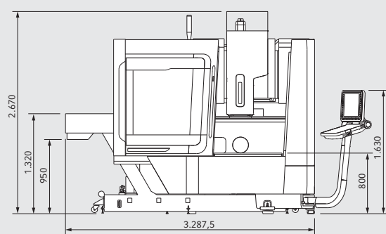
Vista frontal
