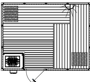
SA-20 / 275 x 210 x 206 / 7 Kw
