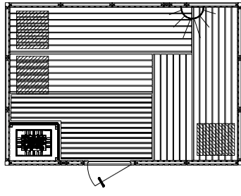
SA-21 / 303 x 210 x 206 / 8 Kw
