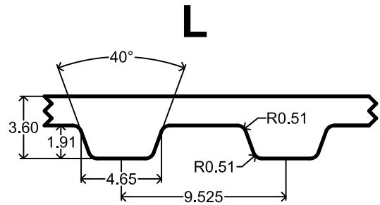
PASO L - 3/8" - 9,525mm
