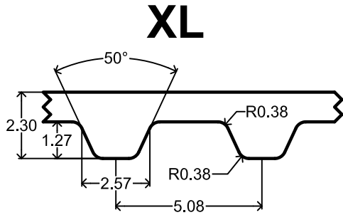
PASO XL - 1/5" - 5,080mm
