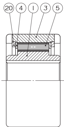
Design/Tipo 242/231
