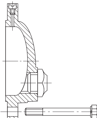
Design/Tipo 220/260 Pg. 13/14
