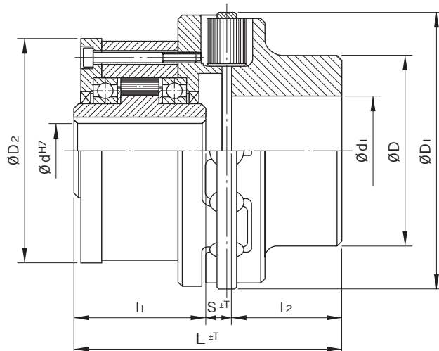
Freewheel + GBN coupling Over size 630/350
