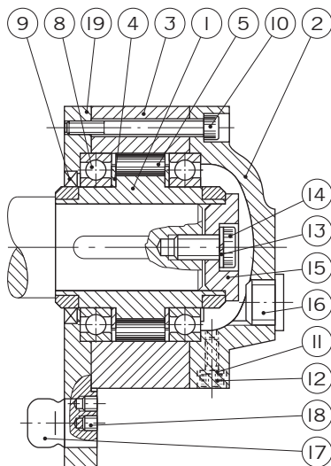
Design/Tipo 242/231
