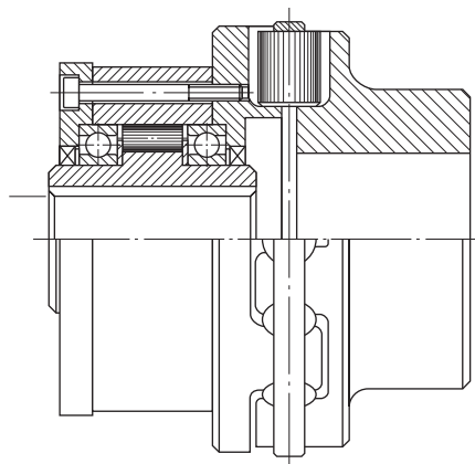
Design/Tipo 228 Pg. 23
