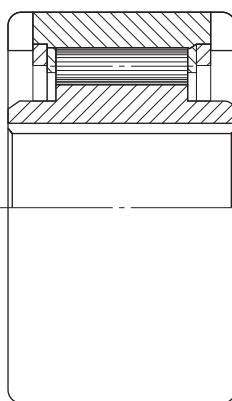
Design/Tipo 242/231 Pg. 11/12
