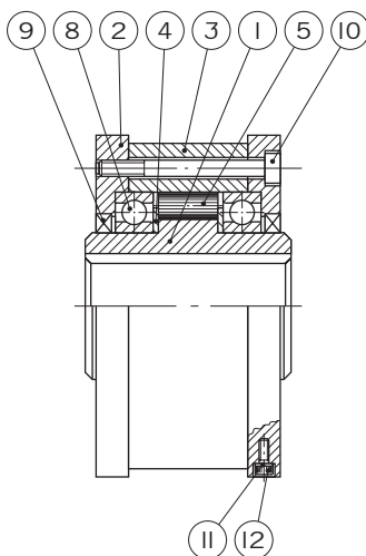
Design/Tipo 221/210
