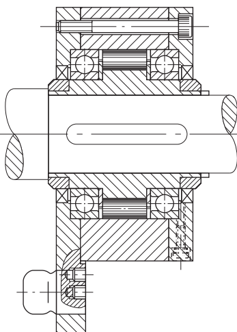
Design/Tipo 257 Pg.18
