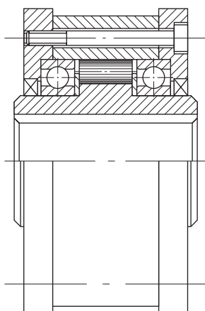
Design/Tipo 221 Pg. 15
