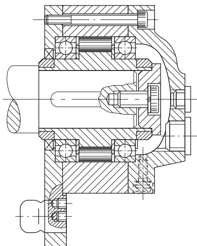
Design/Tipo 255 Pg. 18
