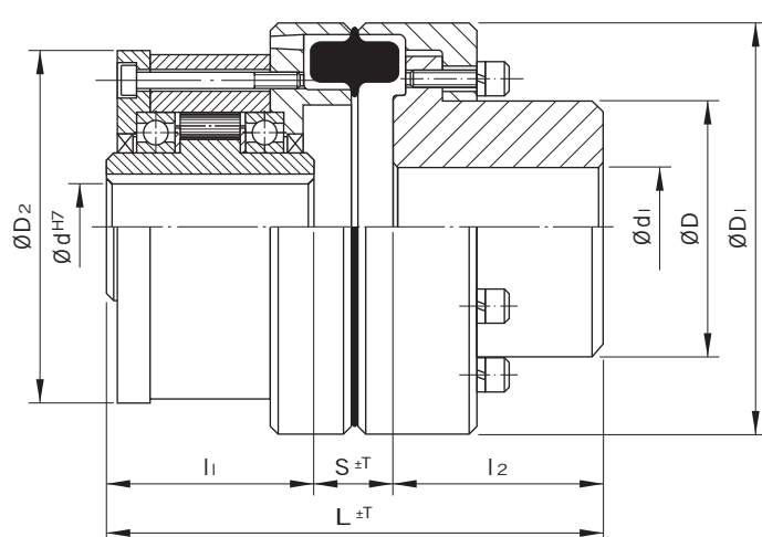
Freewheel 222 + GG coupling up to size 400/330
