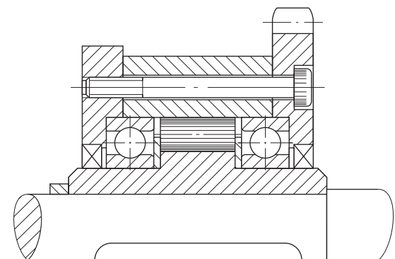
Freewheel design 221 On a through shaft with a chain gear
