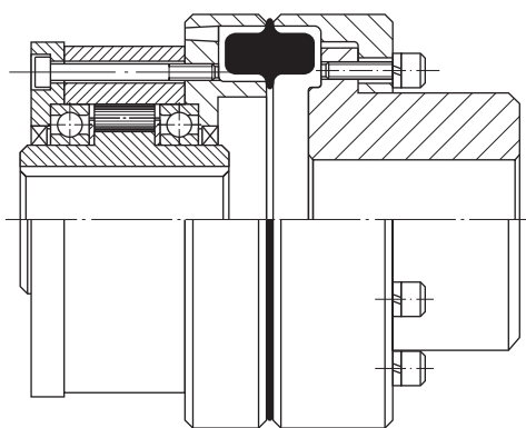
Design/Tipo 228 Pg. 23
