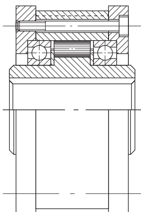
Design/Tipo 210 Pg. 15
