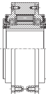
Design/Tipo 261 form 2P Pg. 20
