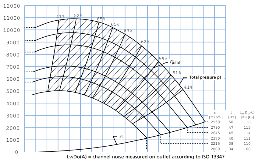
Useful effect and pressure
