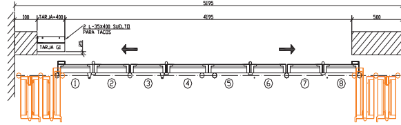
DETALLE GUIA SUPERIOR
