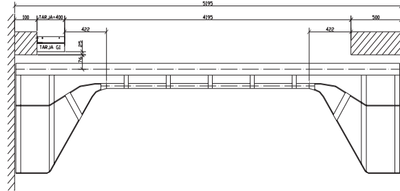
DETALLE GUIA SUPERIOR
