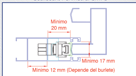
Corredera Perimetral CM75 Perimetral Sliding Windows CM75 Coulissant Perimetral CM75
