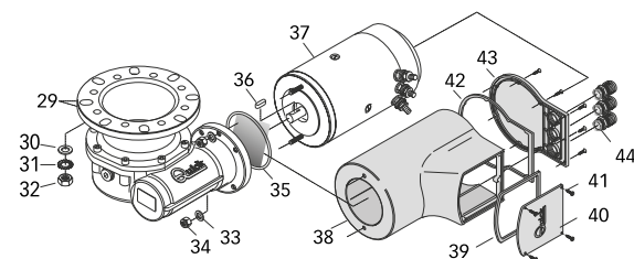
MOTOREDUCTOR 1700W
