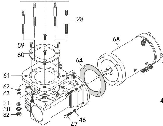
MOTOREDUCTOR 3000W
