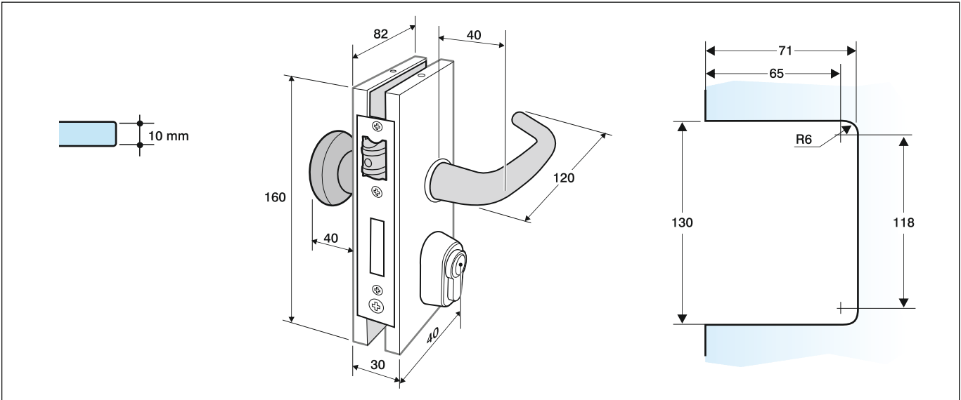
1500/3 Vaivén palanca cilindro pomos oval fijos Rocking latch, lever cylinder and fix oval knobs
