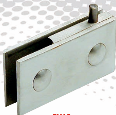
PV10 Pernio vitrina vidrio 10 mm Patch for showcase. Glass thickness: 10mm
