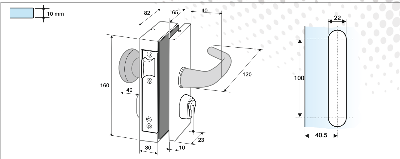
1426 Vaivén palanca cilindro Lock with rocking latch lever and cylinder
