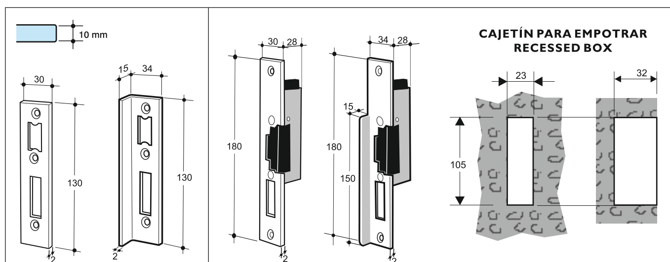
3010 Picaporte eléctrico tope 12V AC con desbloqueo Electric strike box with latch for carpentry, 12V and alternating current (AC) with unlocked with stopper
