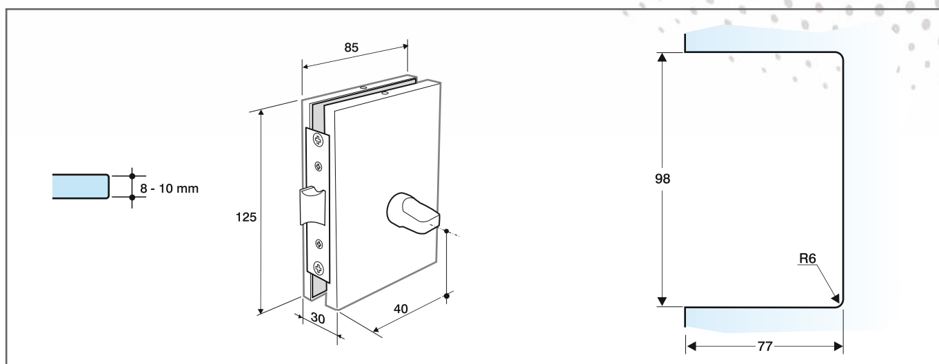
M6000 Picaporte manillas Lock with latch and handle.
