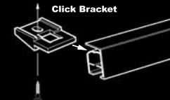
Click Bracket
