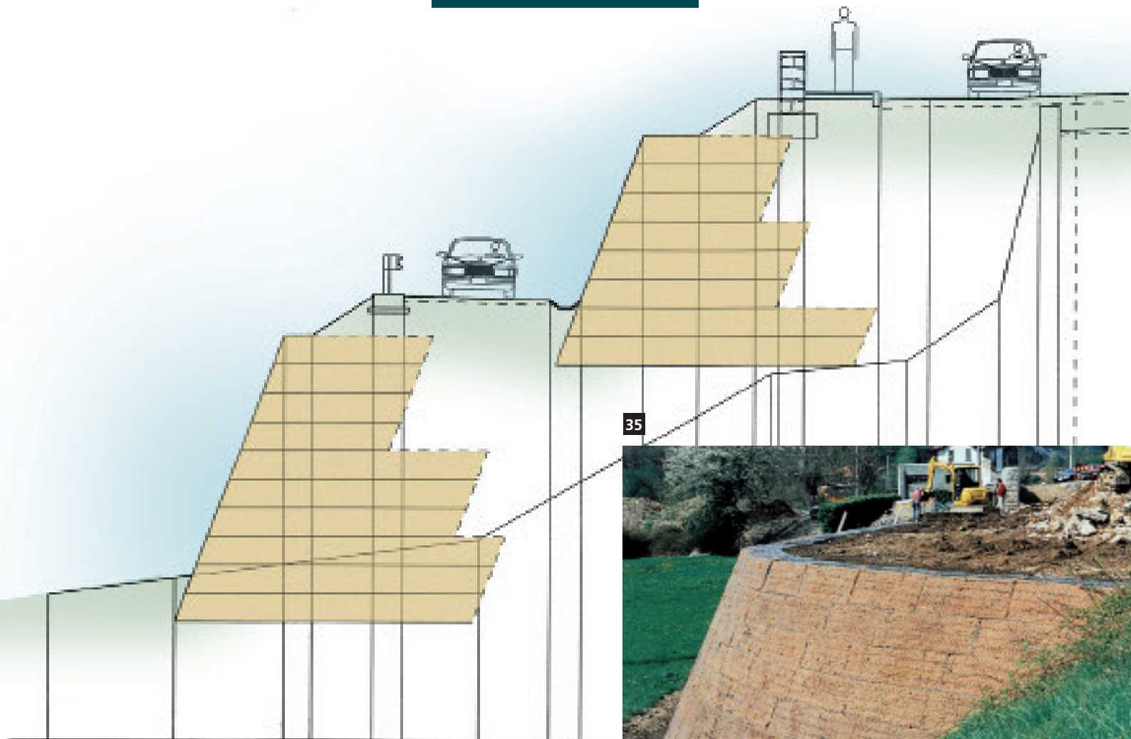
35-36-37. Road restructuring using Green Terramesh®, Valle d'Ogna (BG)-Italy.
