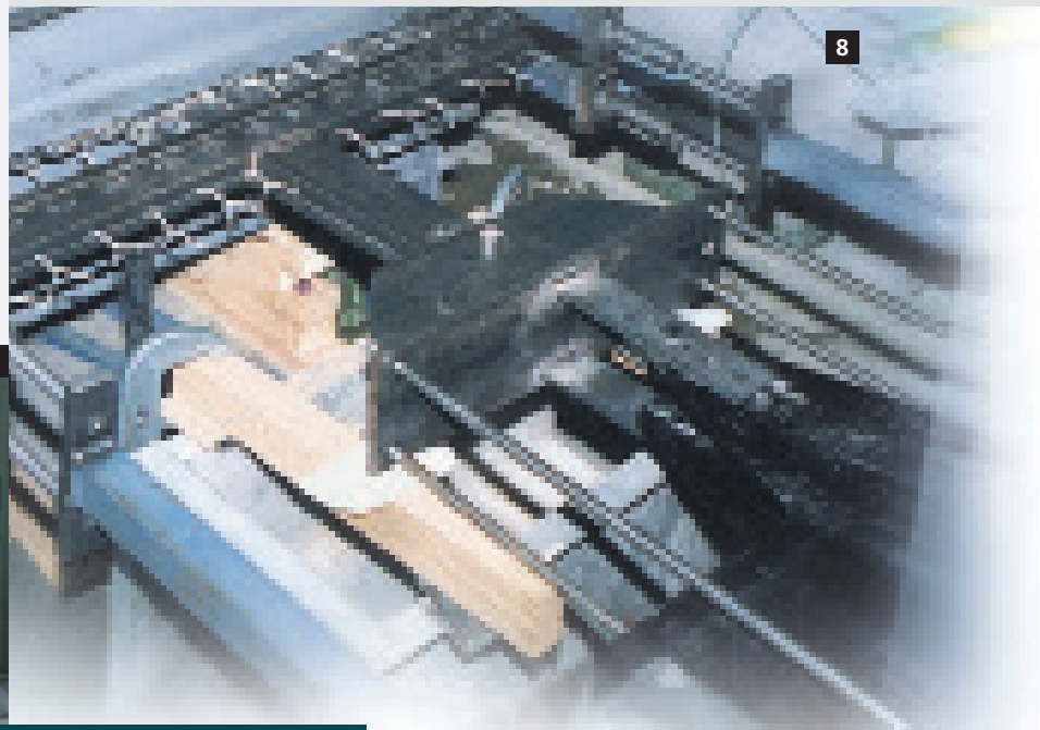
8. Research into the behavior of double twist wire mesh as reinforcement Canberra University, New South Wales-Australia.
