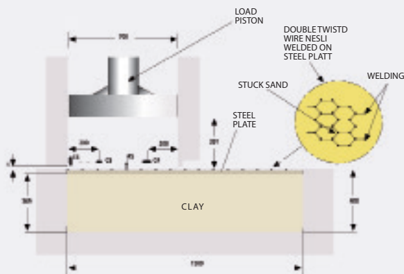
Direct smear box, testing interface soil/mesh
